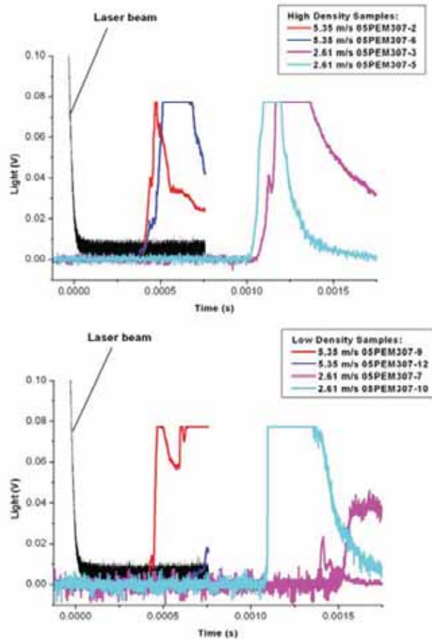
Figure 5.6: Typical times to reaction in stoichiometric nanosize \text{Al} / \text{MoO}_3 samples at indicated drop-weight impact velocity and a high green density (up) or low density (down). Experiments are performed in duplicate.
