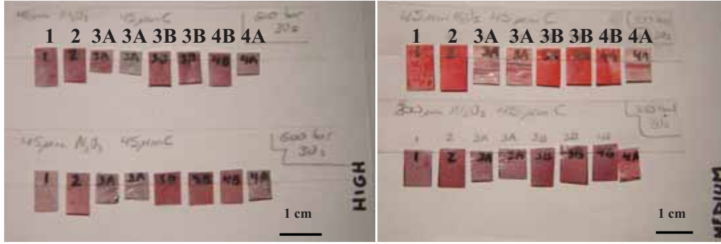
Figure 2.4: Sensor films after removal from the PTM. Left: sensors type high (49-120 MPa) after pressing at 105 MPa (45 µm alumina); Right: sensors type medium (9.7-49 MPa) after pressing at 55 MPa (300 µm alumina).
