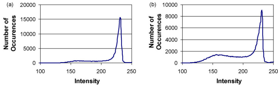
Fig. 6. ImageJ analysis of pressure film results for bare steel with (a) 5 PMMA balls and (b) 15 PMMA balls.
