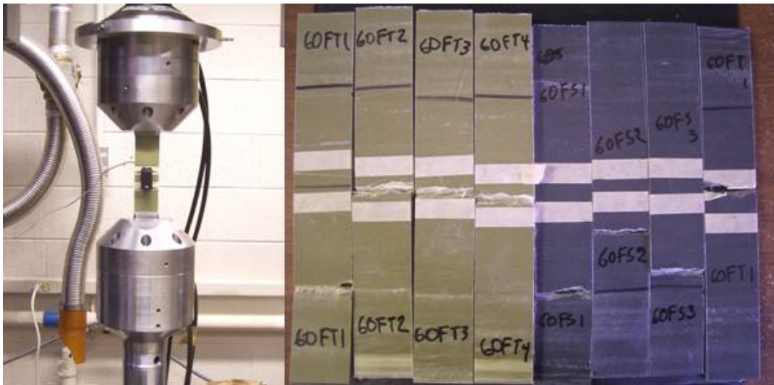
Figure 6.5 Transverse tension fatigue test with plate samples
