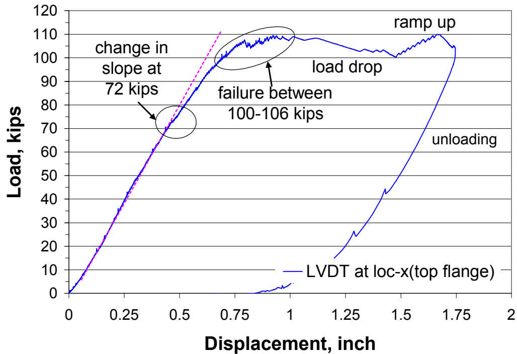
Figure 6.3 Load vs. displacement behavior at top flange (location-L in Figure 6.2)
