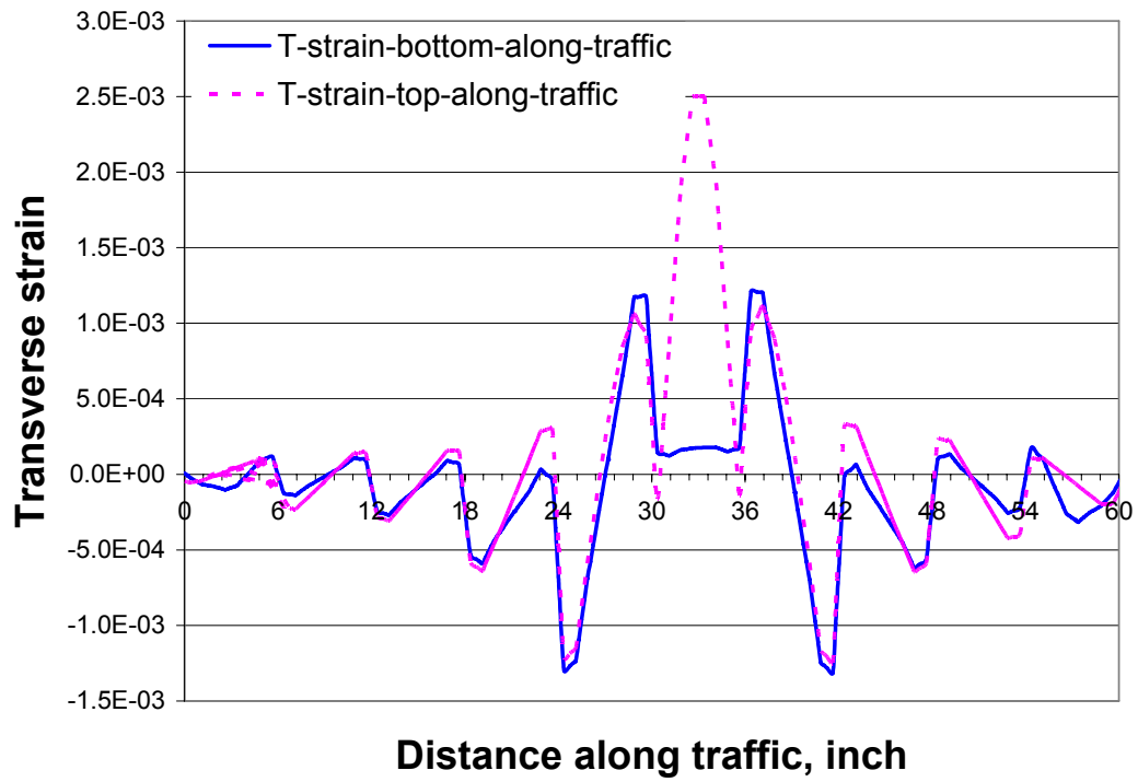
Figure 5.22 Local transverse strain distribution along traffic direction (vertical grid lines also represent web locations at 6 inch spacing)
