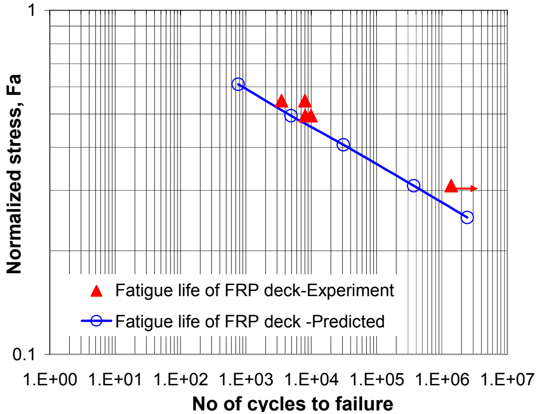
Figure 6.16 Predicted Life of FRP bridge deck
