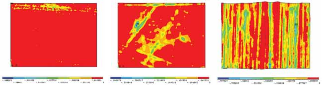
Figure 2-10: Contact Gap (µm): 2L Sample (left), 4L (middle), 8L (right)
