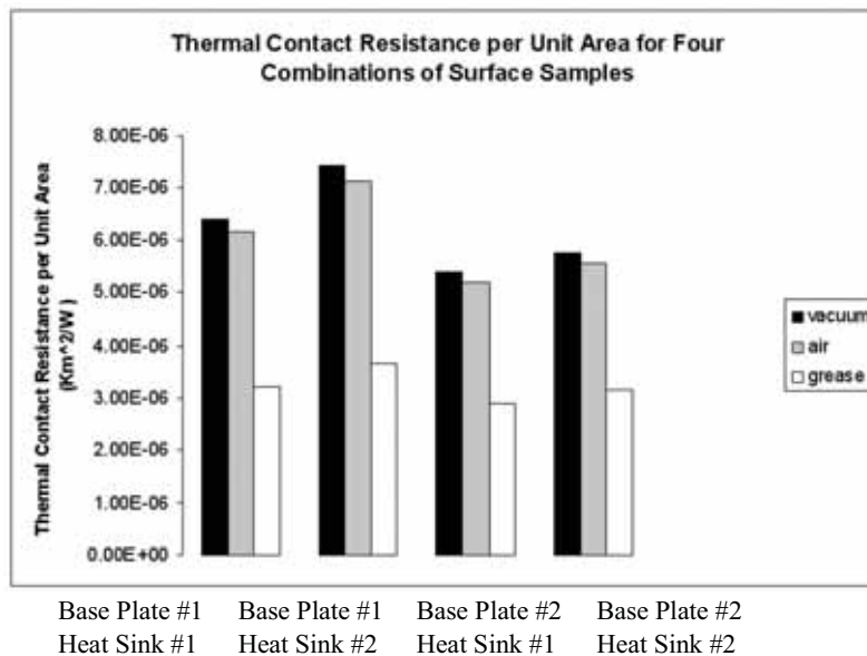
Figure 5-6: Micro Scale TCR vs. Various Combinations of Surface Samples ( P/E = 3.23e-4 )
