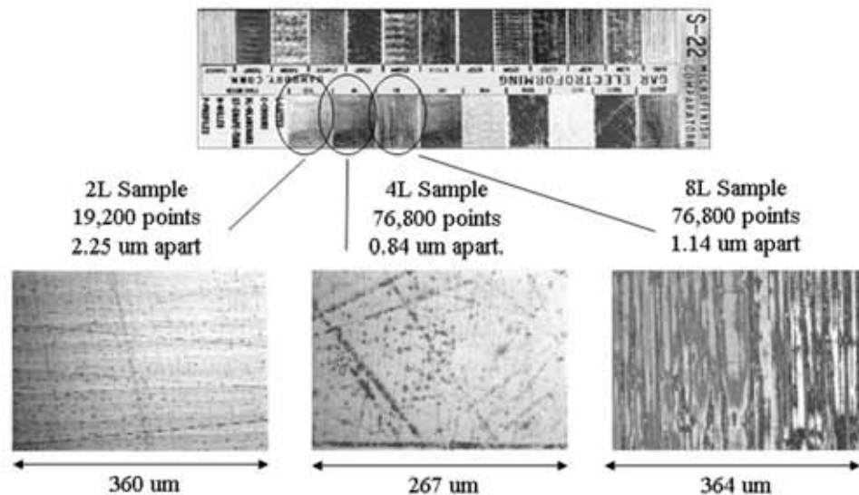
Figure 2-6: Surface Comparator
