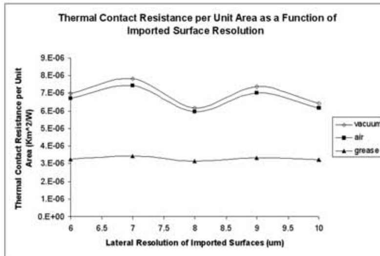
Figure 5-7: Micro Scale TCR vs. Imported Surface Resolution ( P/E = 3.23\text{e-}4 )
