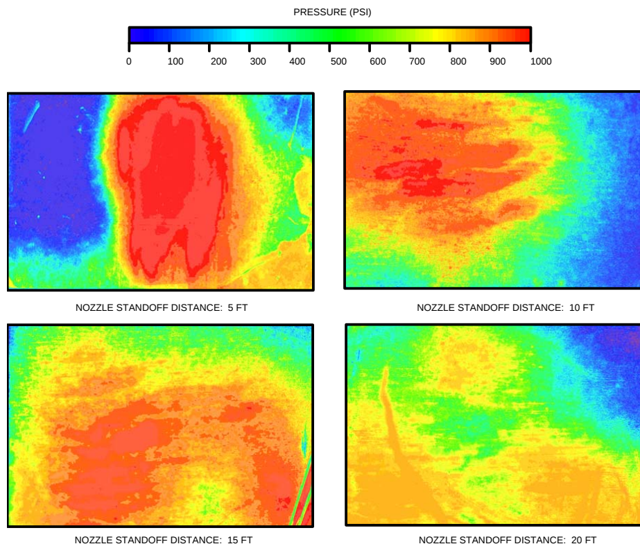
Figure 4.8.3: Exposed Low Pressurex® (0 – 1000 psi) film contours of total impact pressure for 5, 10, 15, and 20 foot standoff distances from the nozzle.
